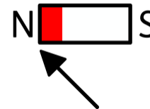
north pole
