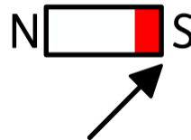
south pole
