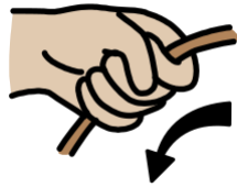
pull
