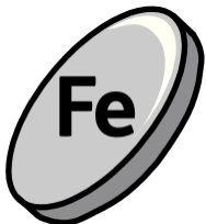
iron
