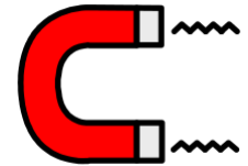
magnet
